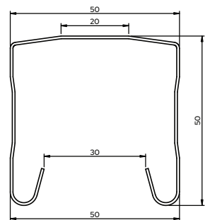
0.8 COLORBOND FENCE RAIL PROFILE VIEW
